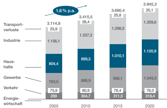
Prognose Stromverbrauch EU-27 2020 (in TWh)
